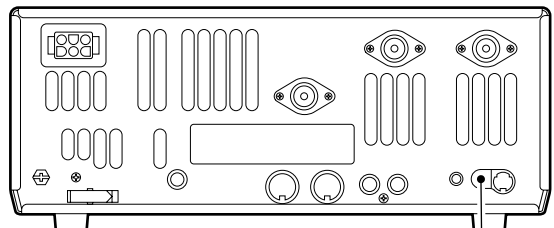
EXTERNAL SPEAKER
