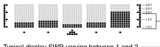
Typical display SWR varying between 1 and 2, full scale up to SWR 4.0:1.
